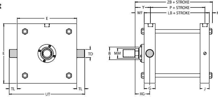
STYLE ER—Trunnion Mount Head End (NFPA Mounting Style MT1)
