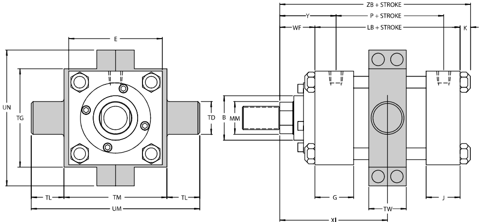
STYLE E—Intermediate Trunnion Mount (NFA Mounting Style MT4)
