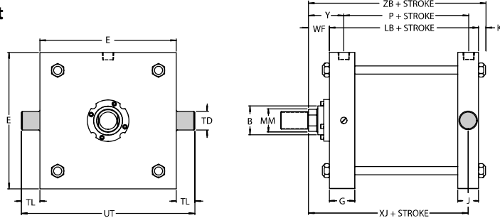
STYLE EB—Trunnion Mount Cap End (NFPA Mounting Style MT2)
