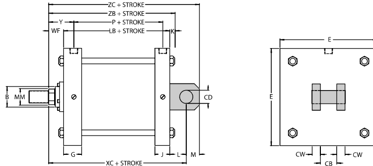
STYLE G—Cleviss Mount (NFPA Mounting Style MP1)
