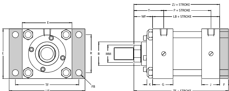
STYLE A—Rectangular Flange Mount Cap End (NFPA Mounting Style MF2)
