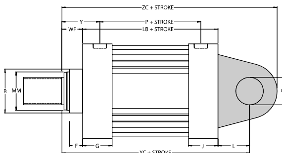
STYLE G—Clevis Mount (NFPA Mounting Style MP1)
