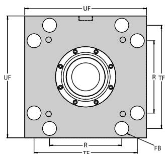
STYLE QQ—Square Head End Mount (NFPA Mounting Style ME3)
