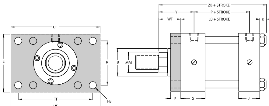
STYLE B—Rectangular Flange Mount Head End (NFPA Mounting Style MF1)
