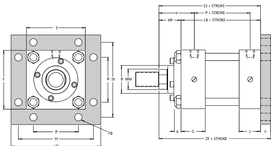
STYLE AA—Square Flange Mount Cap End (NFPA Mounting Style MF6)
