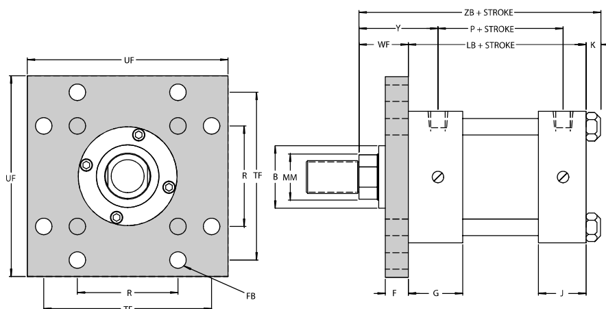
STYLE BB—Square Flange Mount Head End (NFPA Mounting Style MF5)
